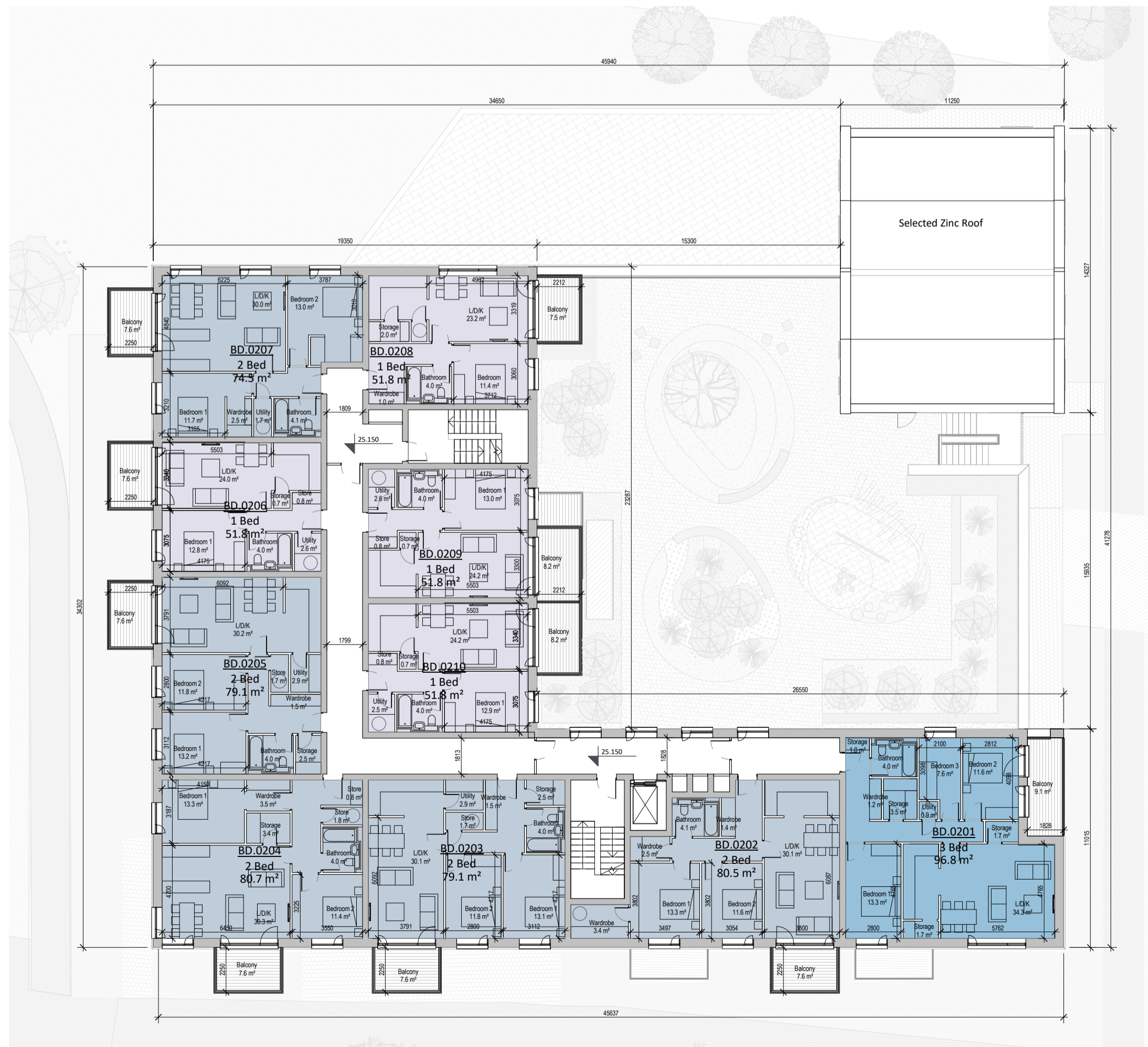
3 Block D - Level 02 1:200
